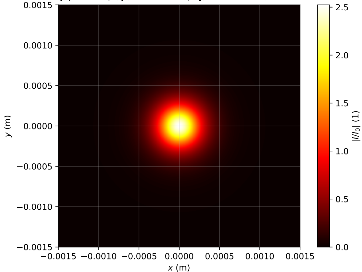
Intensity profile I(x, y, z = 2.786m)/I_0 , Pin=1.0Pcr, artificial time
